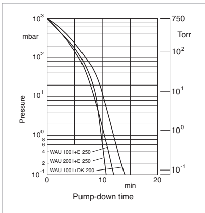
Pump-down time diagram for a 10 \text{ m}^3 tank at 50 Hz
