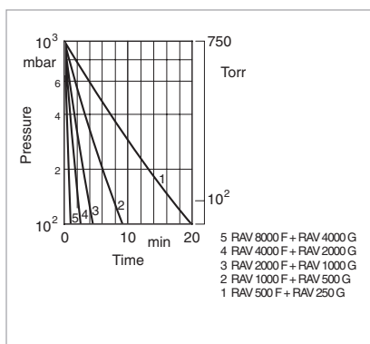
Pump-down time diagram for a 50 m 3 tank for RAV F+G at 50 Hz
