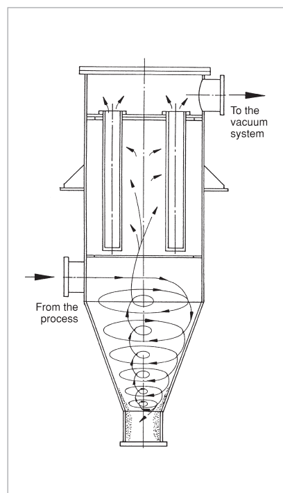
Diagrammatic section through a dust separator
