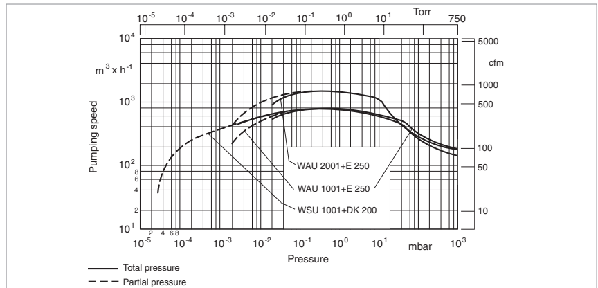
Pumping speed diagram at 50 Hz
